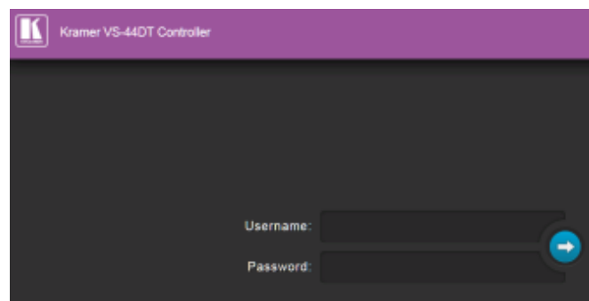
Figure 21: Login Page
