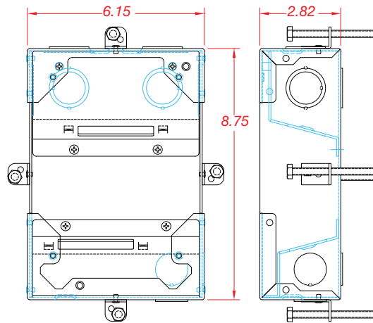
3"-DEEP BOX
