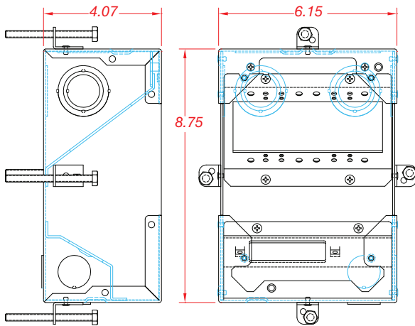
4"-DEEP BOX
