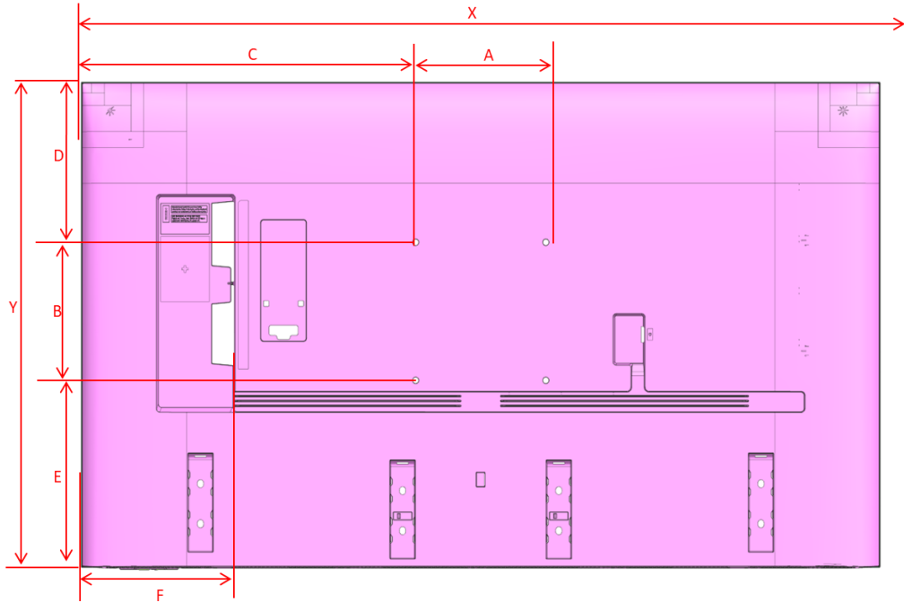
QN85D Cover and Rear-View Dimensions
