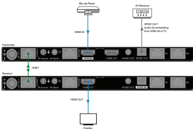
Figure 3: To extract TX HDMI IN audio
