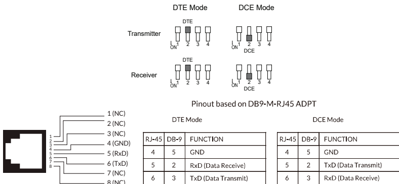
Figure 6: RS-232 Modes and Connections
