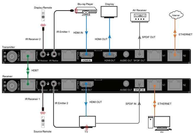
Application Diagram 2
