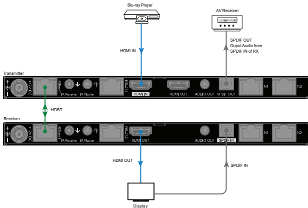
Figure 2: To return SPDIF inserted audio
