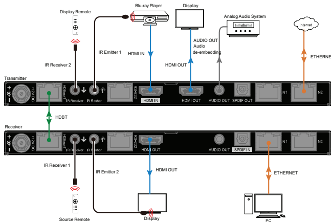
Application Diagram 1
