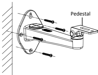
Figure 2-5 Install the Wall Mounting Bracket
